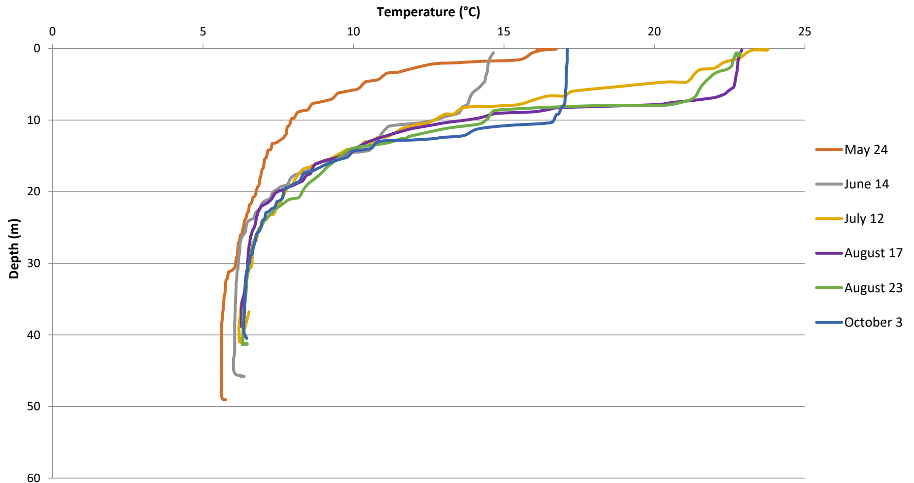
MLK-02: Depth vs. Temperature May-October 2016
